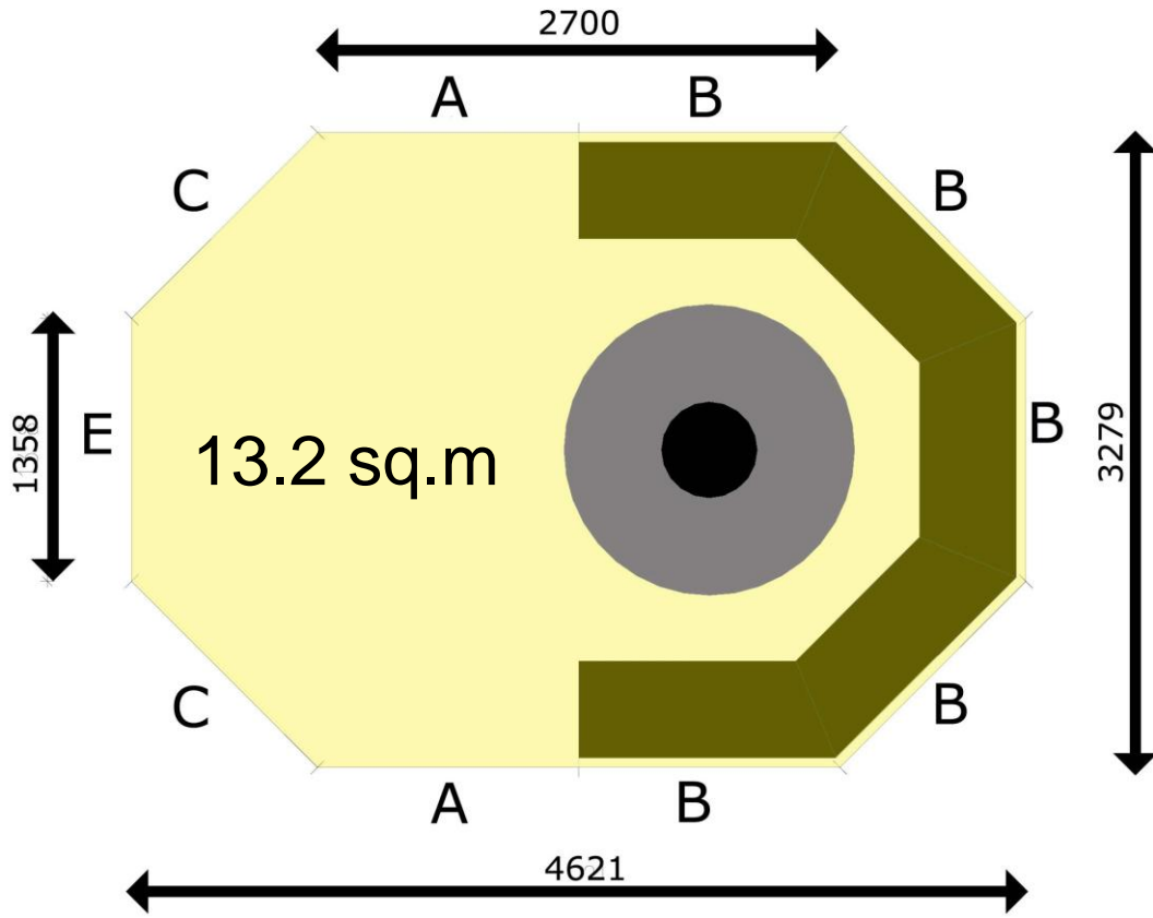
Garden House Max Floor Plan
